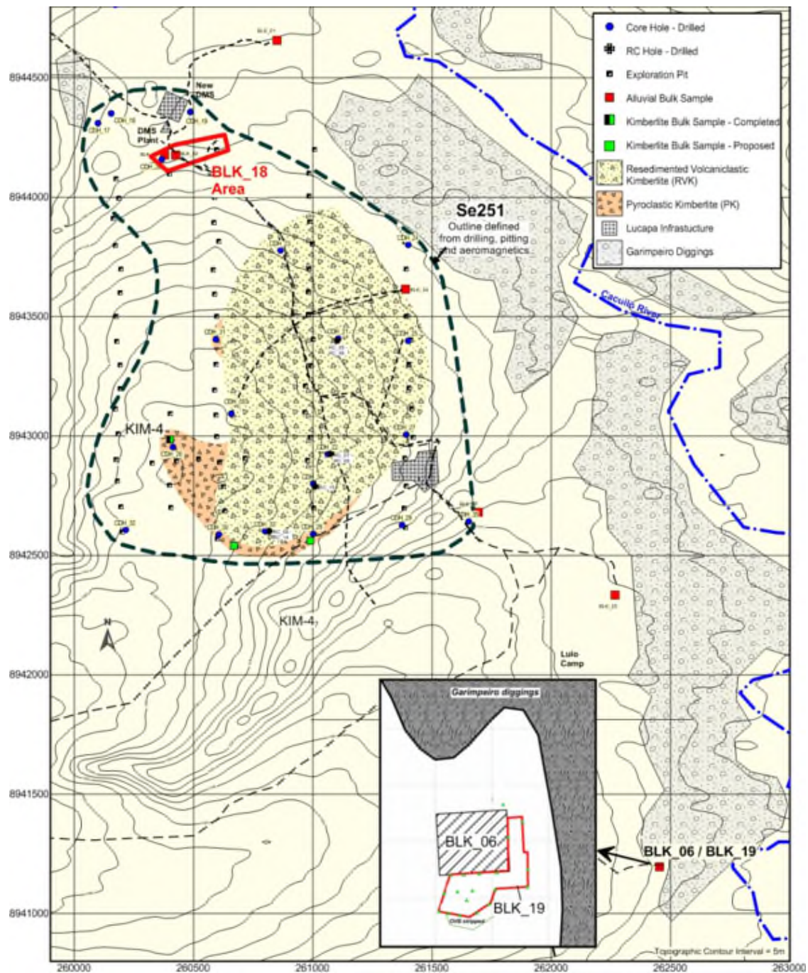
Figure 1 – Location of bulk samples in relation to Se251 kimberlite pipe
