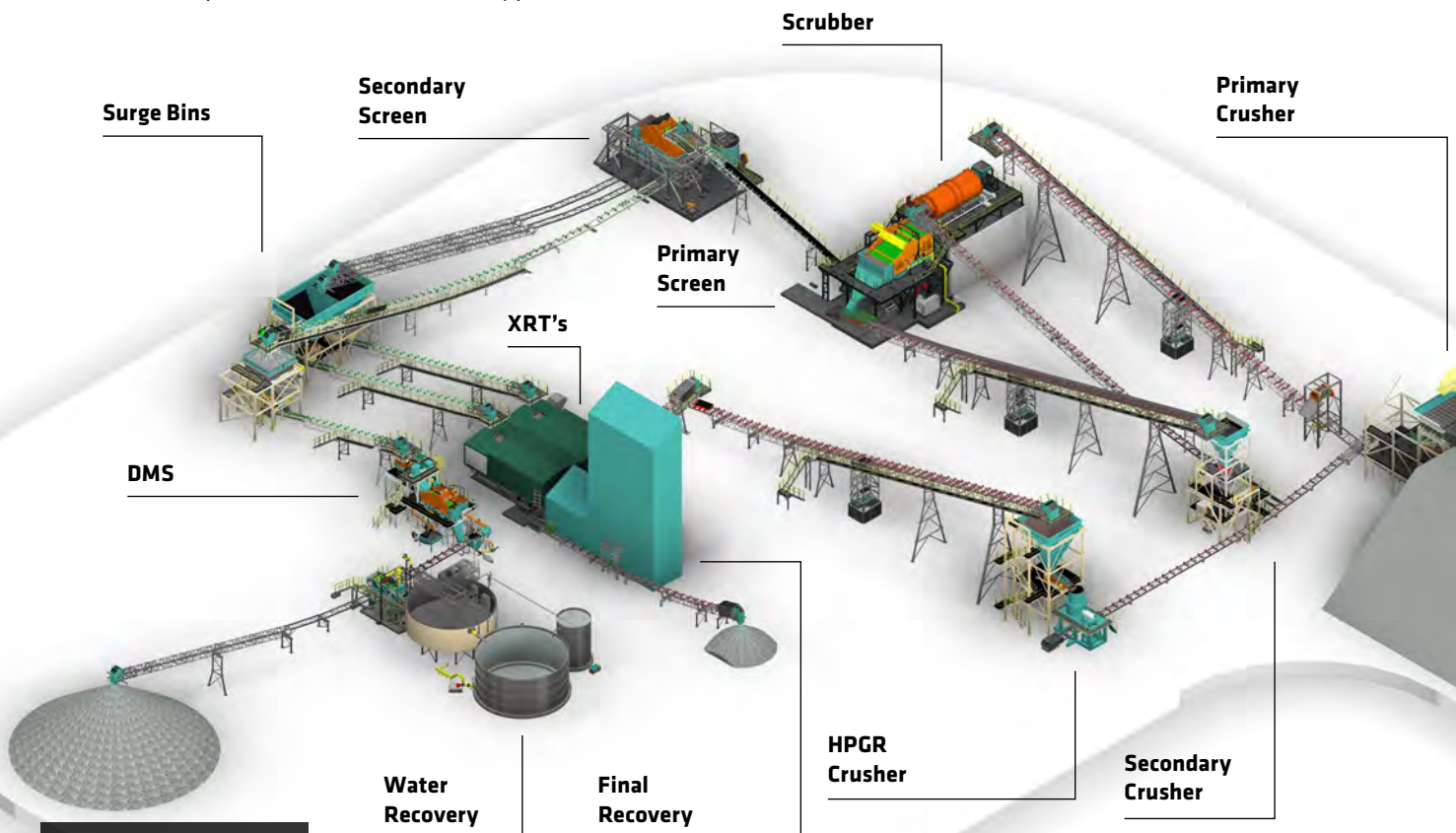
Figure 8: Merlin plant schematic
