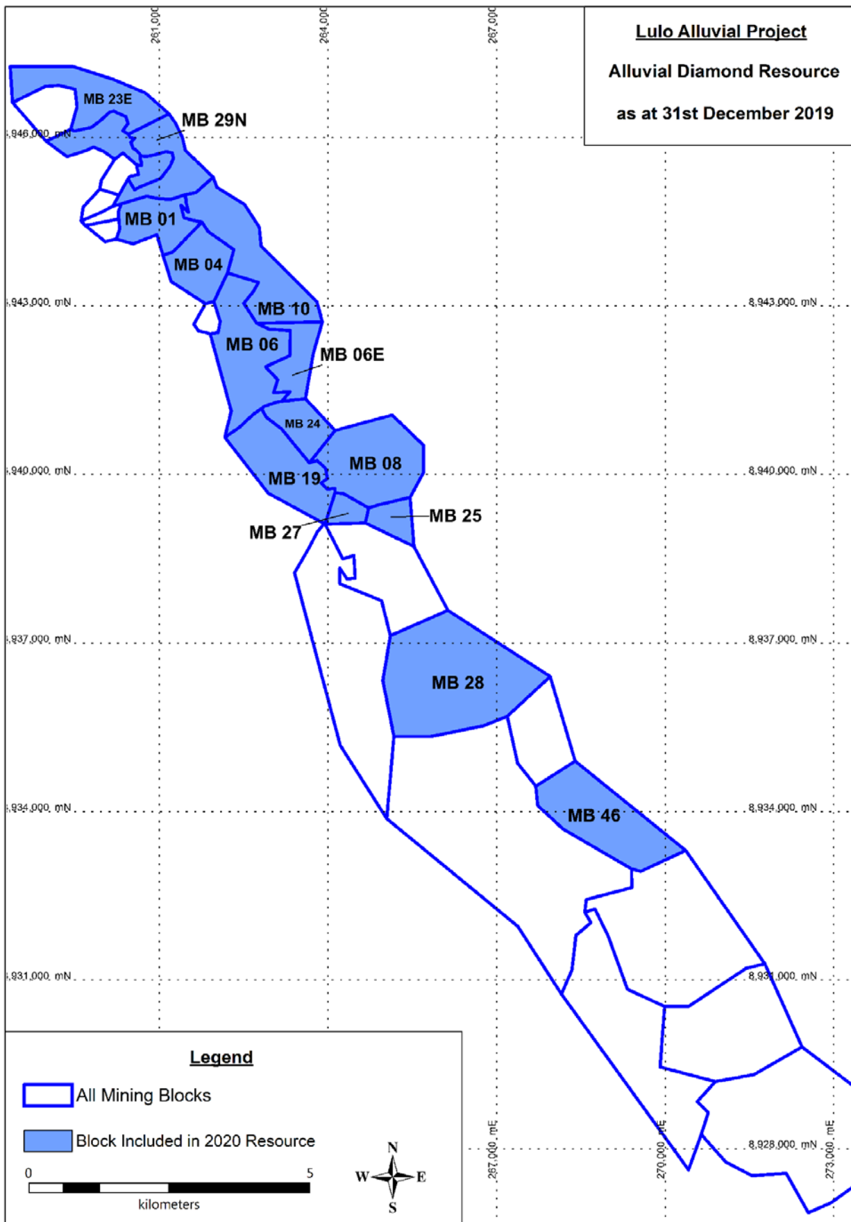
Appendix 2: Map of the alluvial Mining Blocks included in the Lulo Alluvial Diamond Resource
